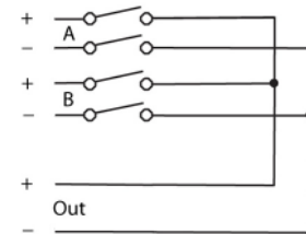
DigESwitch Differential Mux-(one channel shown)
