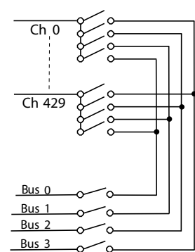
DigESwitch 4-Bus Matrix
