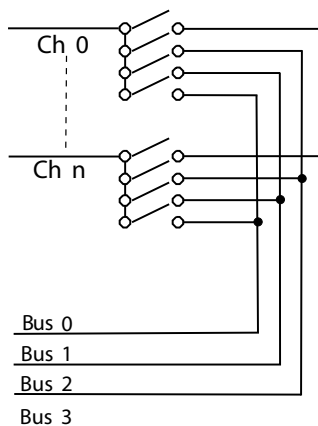
(n + 1) x 4 Matrix
