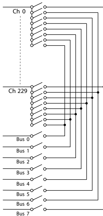
DigESwitch 8-Bus Matrix
